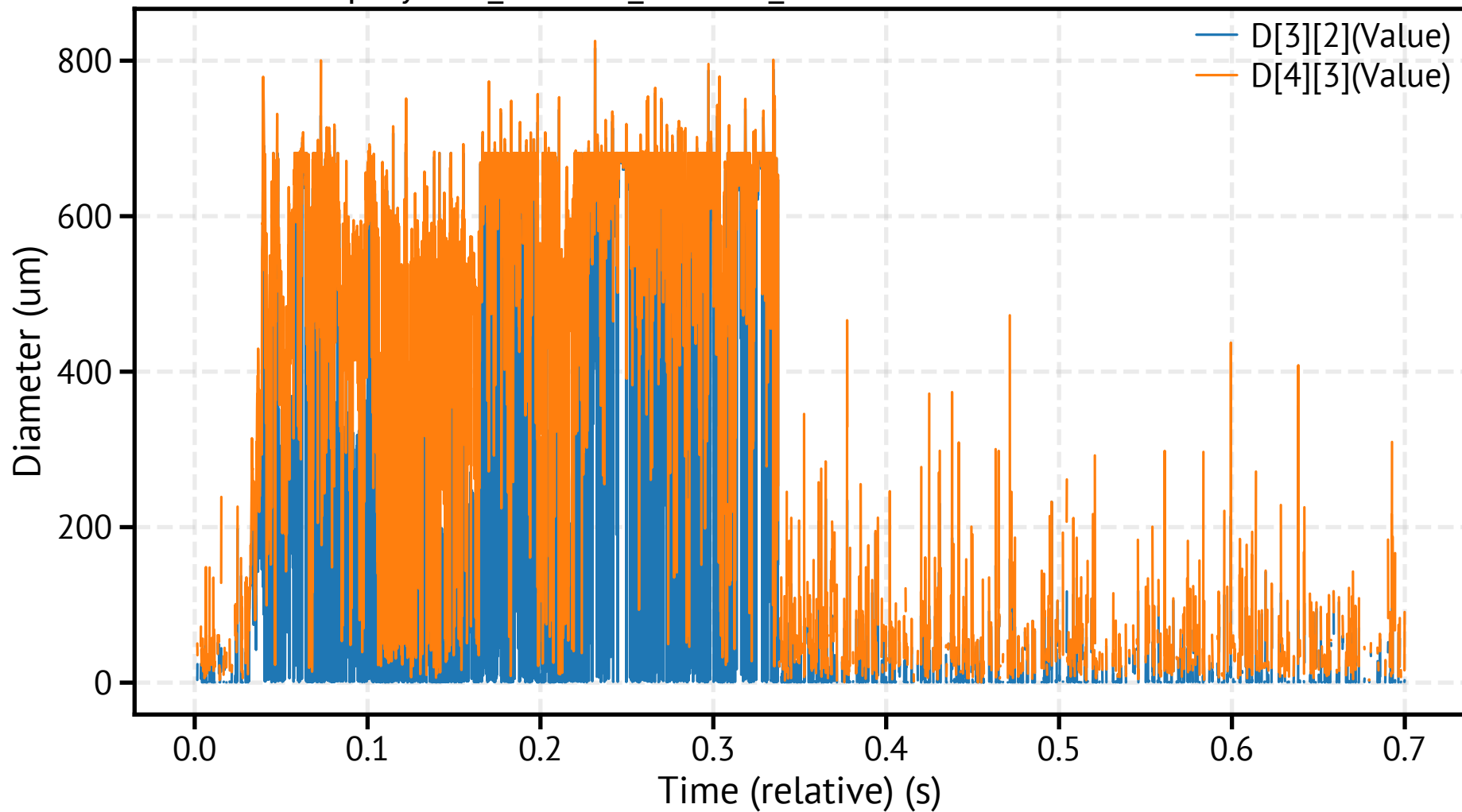
spraytec2_260318_135416_796600.csv - Mean Diameters
