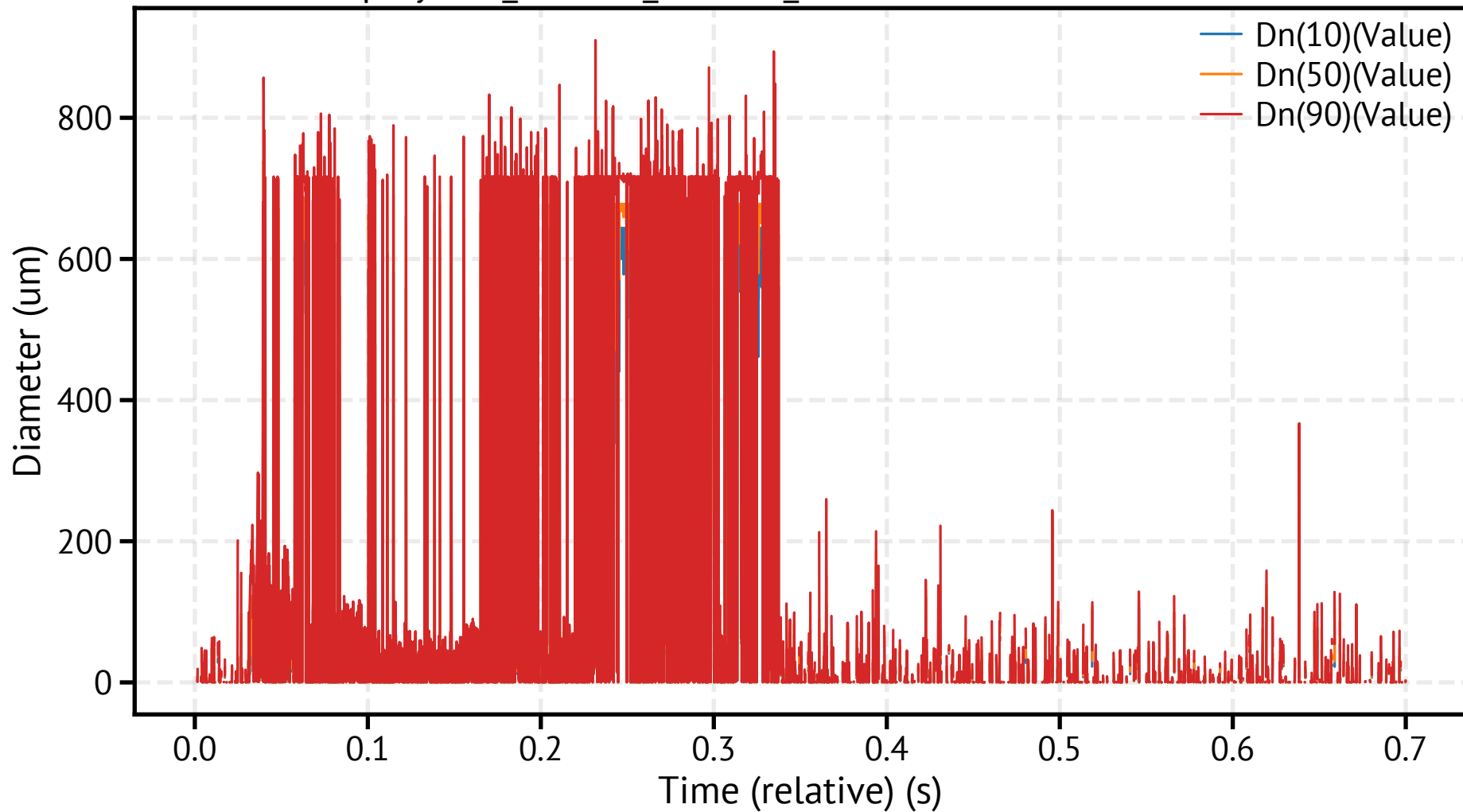
spraytec2_260318_135416_796600.csv - Dn Percentiles
