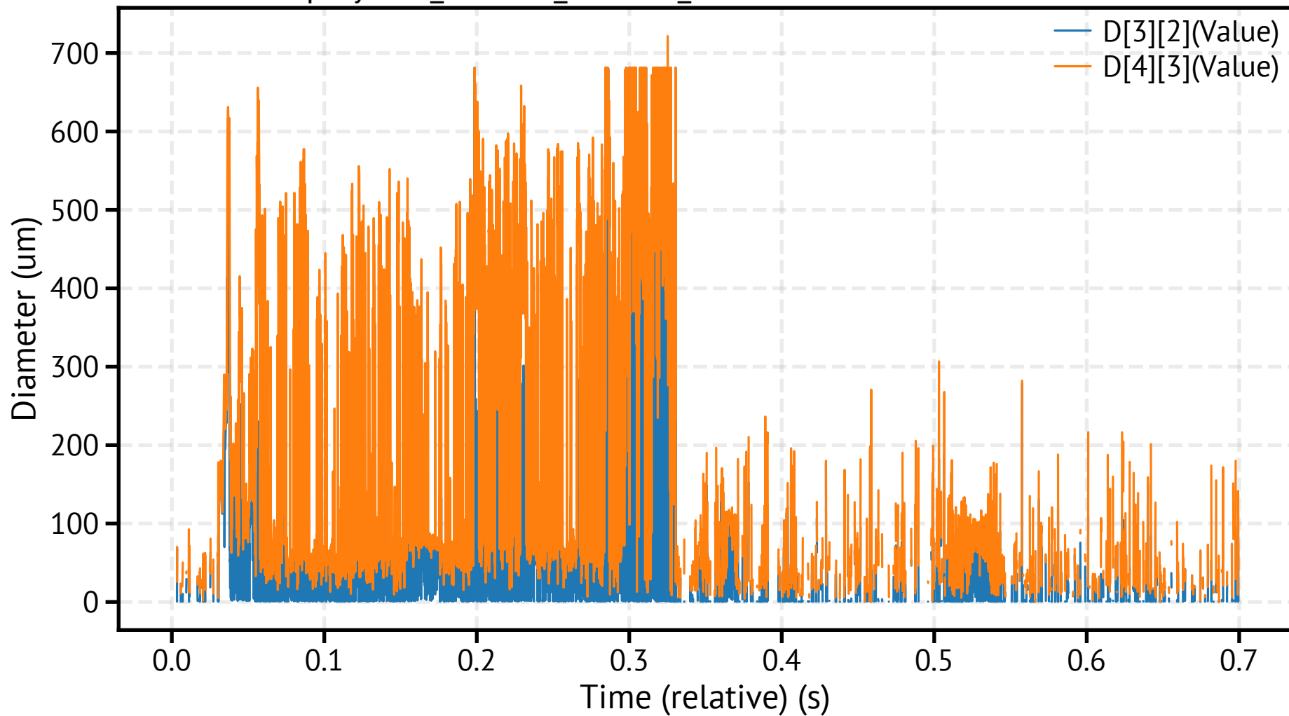
spraytec3_260318_135514_493300.csv - Mean Diameters
