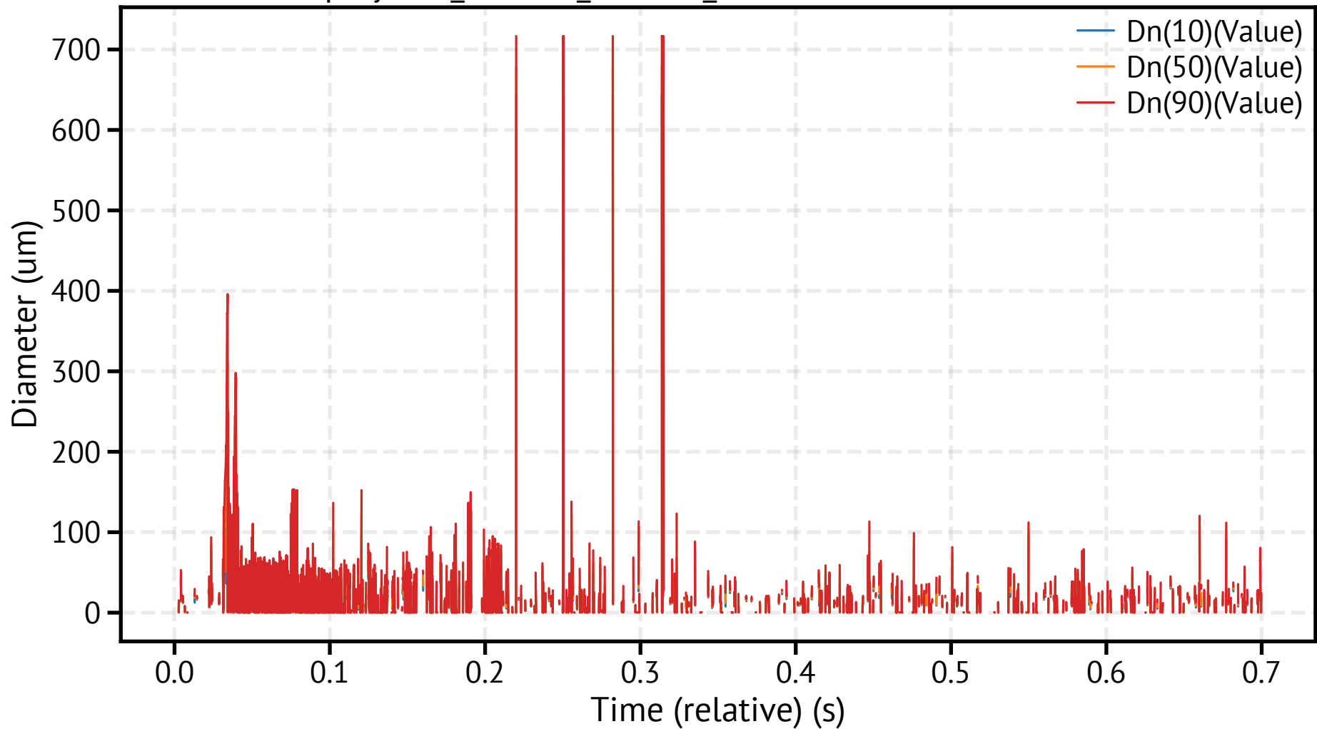
spraytec7_260318_135905_017600.csv - Dn Percentiles
