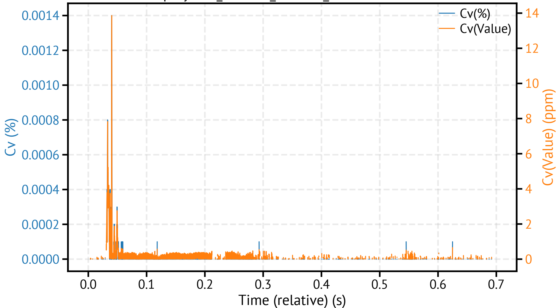
spraytec9_260318_140100_404400.csv - Cv
