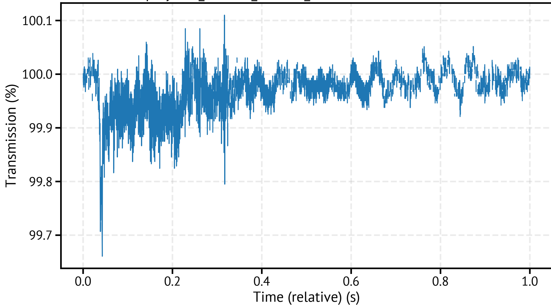
spraytec2_260310_133430_575700.csv - Transmission
