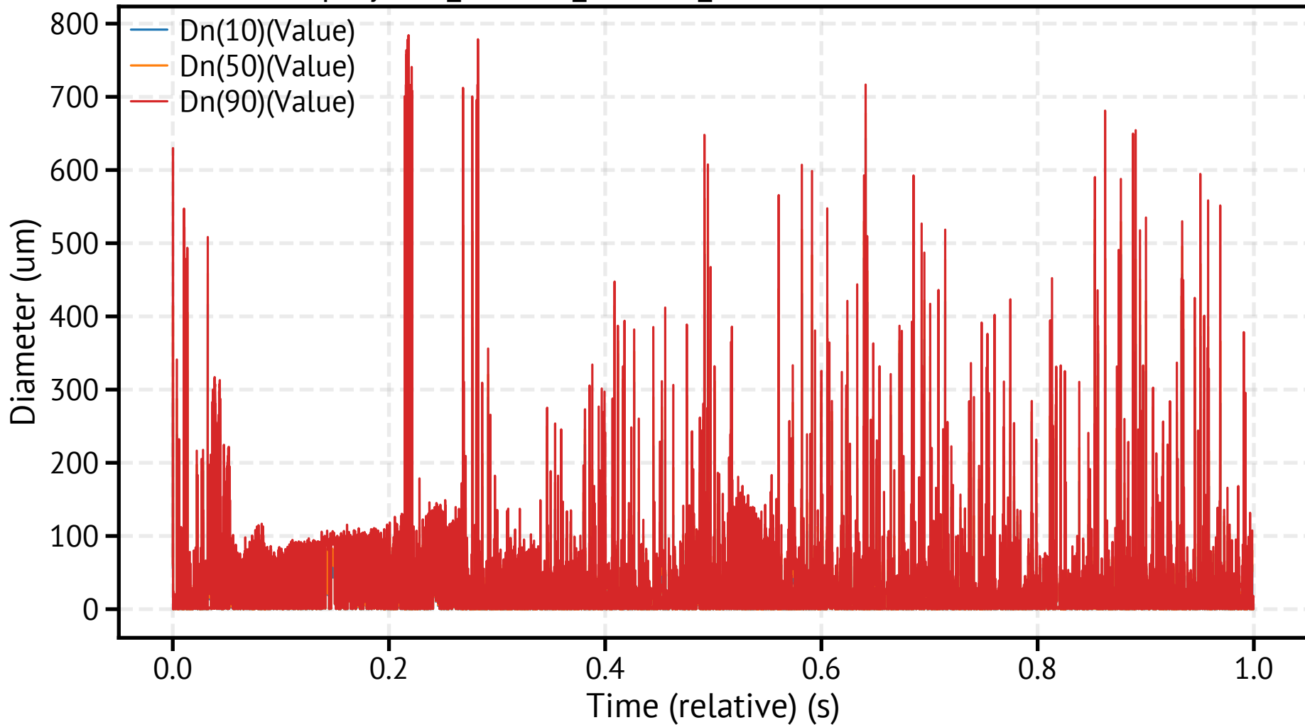
spraytec1_260310_142607_645400.csv - Dn Percentiles
