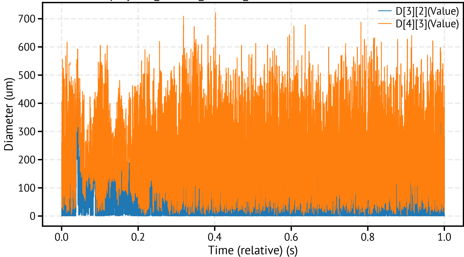
spraytec3_260310_142703_308500.csv - Mean Diameters
