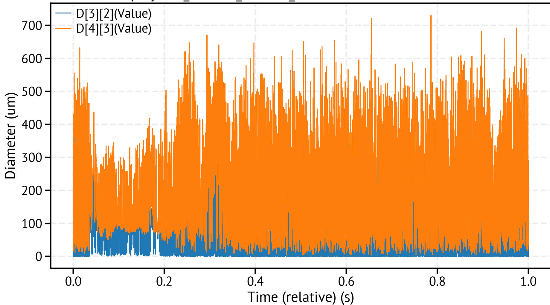
spraytec4_260310_142731_173600.csv - Mean Diameters
