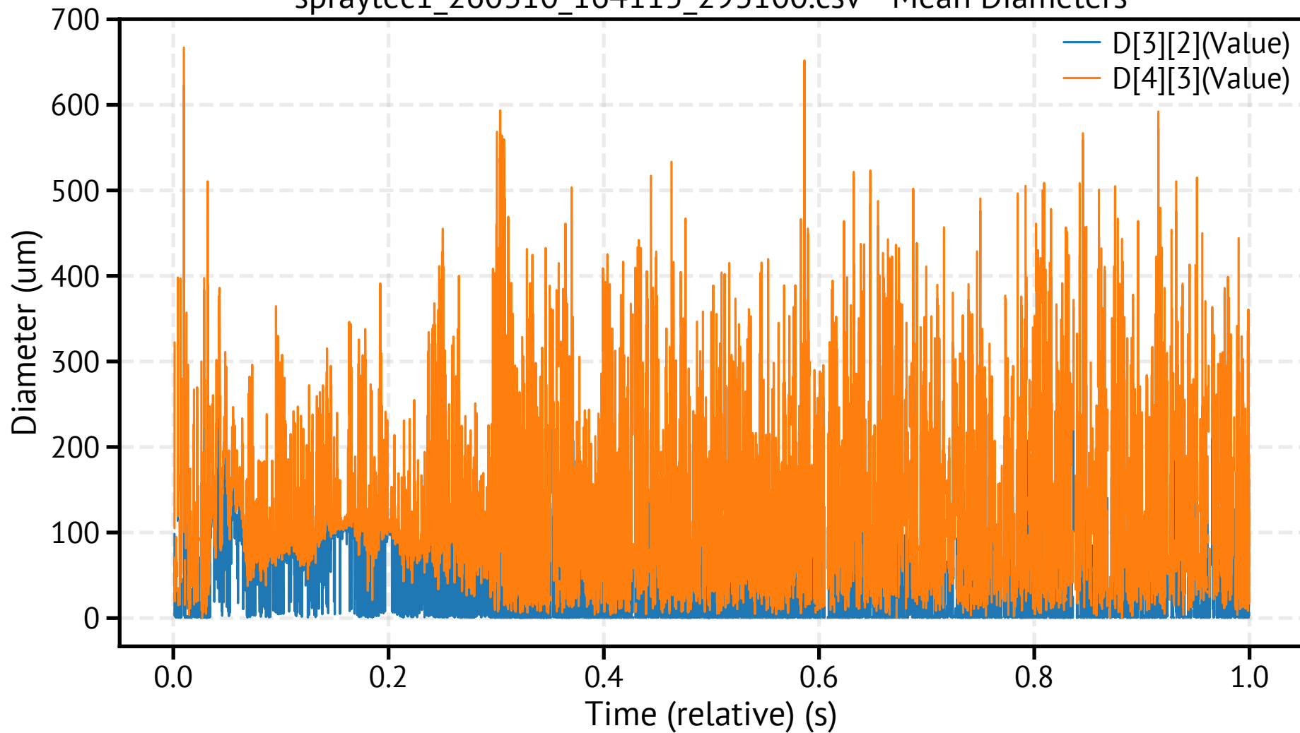
spraytec1_260310_164115_293100.csv - Mean Diameters
