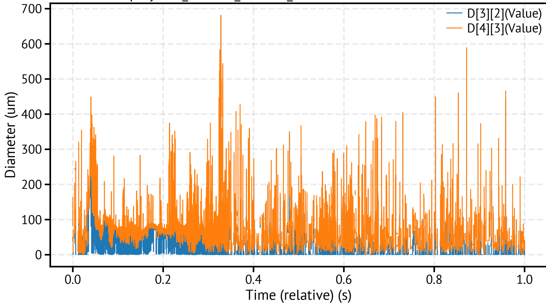
spraytec3_260310_164211_072400.csv - Mean Diameters
