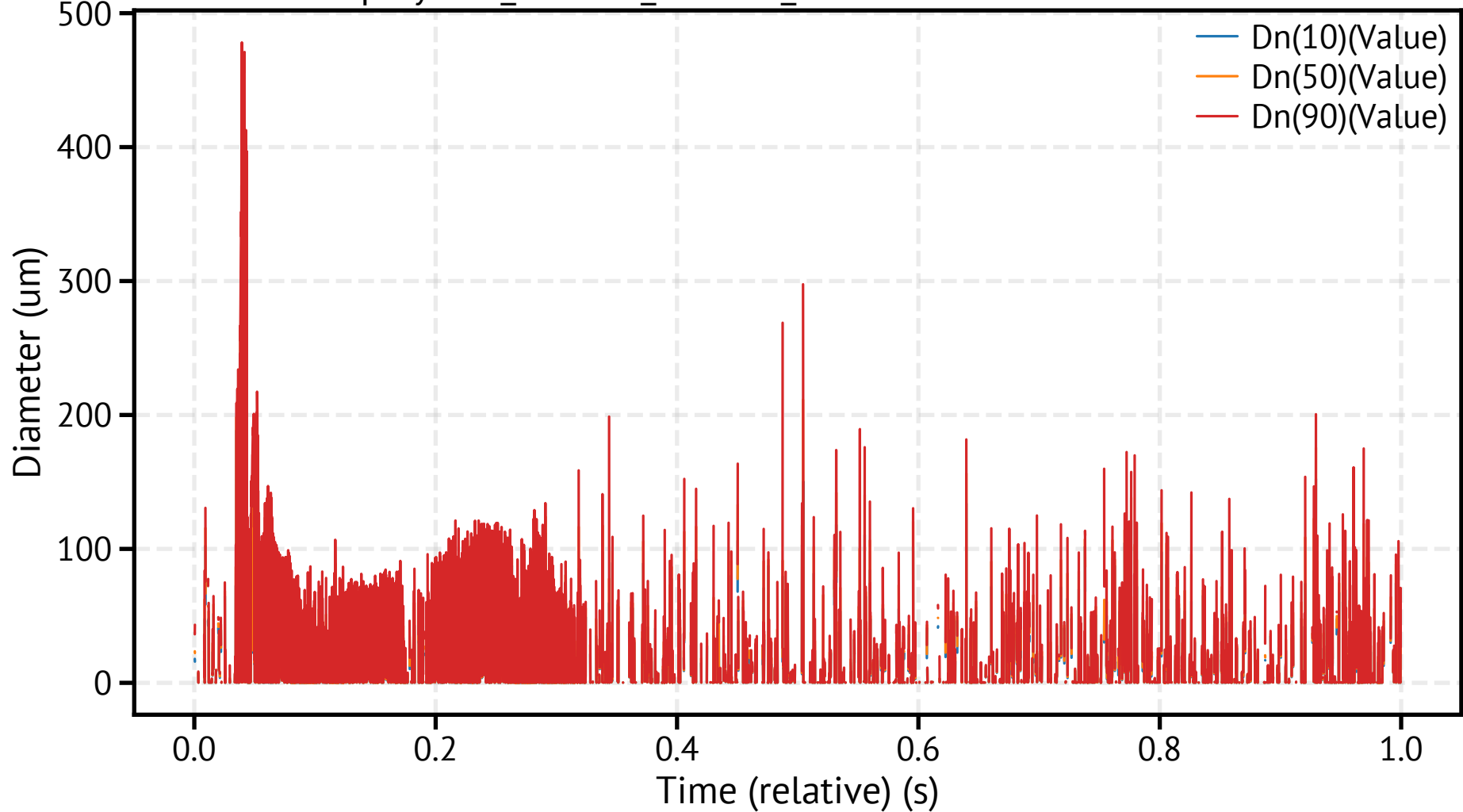
spraytec5_260310_164306_769500.csv - Dn Percentiles
