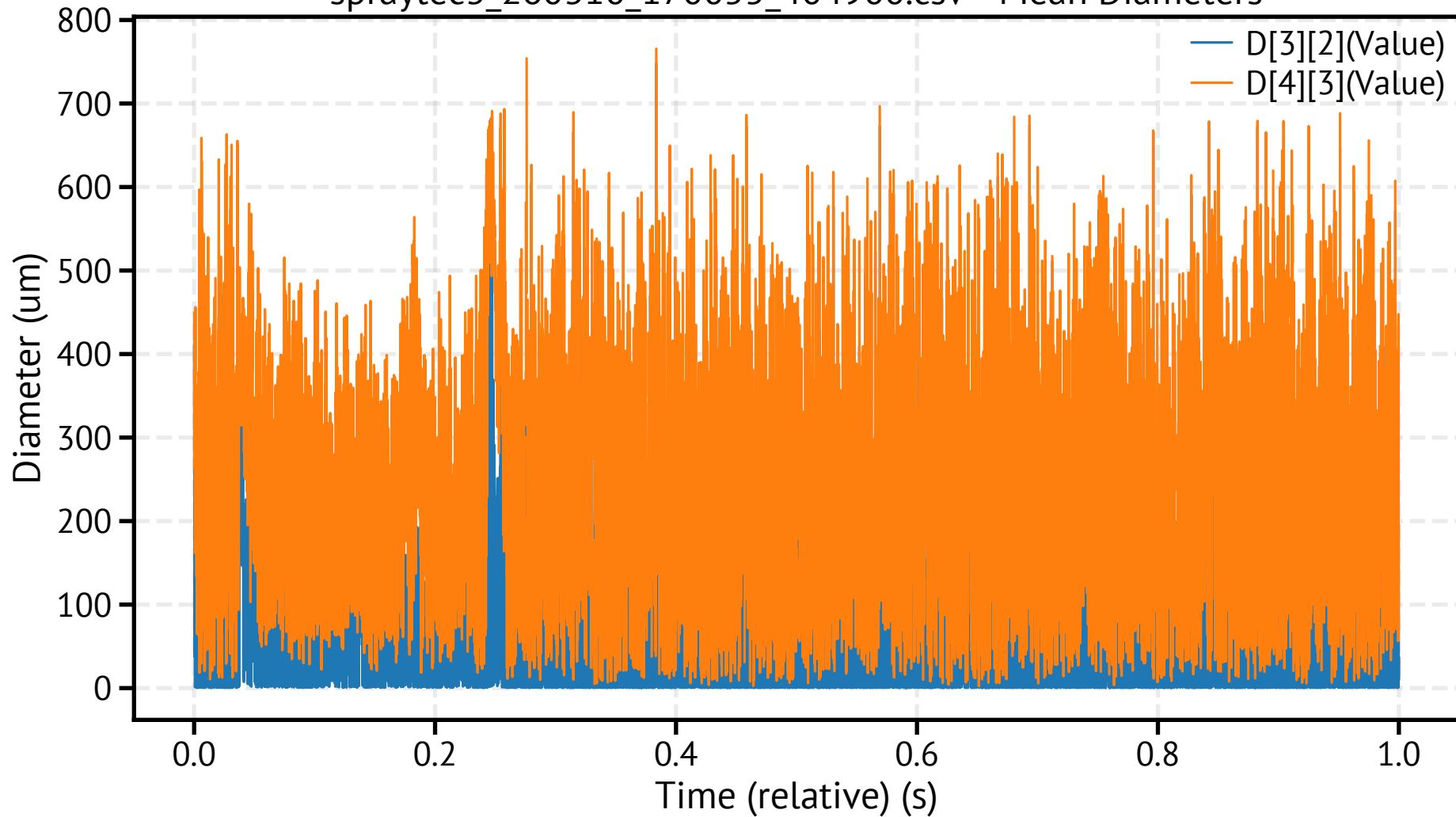
spraytec3_260310_170055_404900.csv - Mean Diameters
