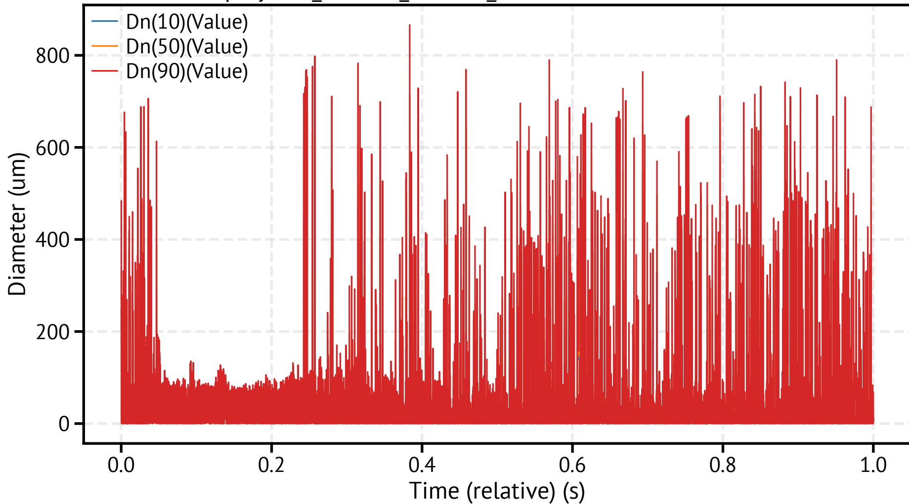
spraytec3_260310_170055_404900.csv - Dn Percentiles
