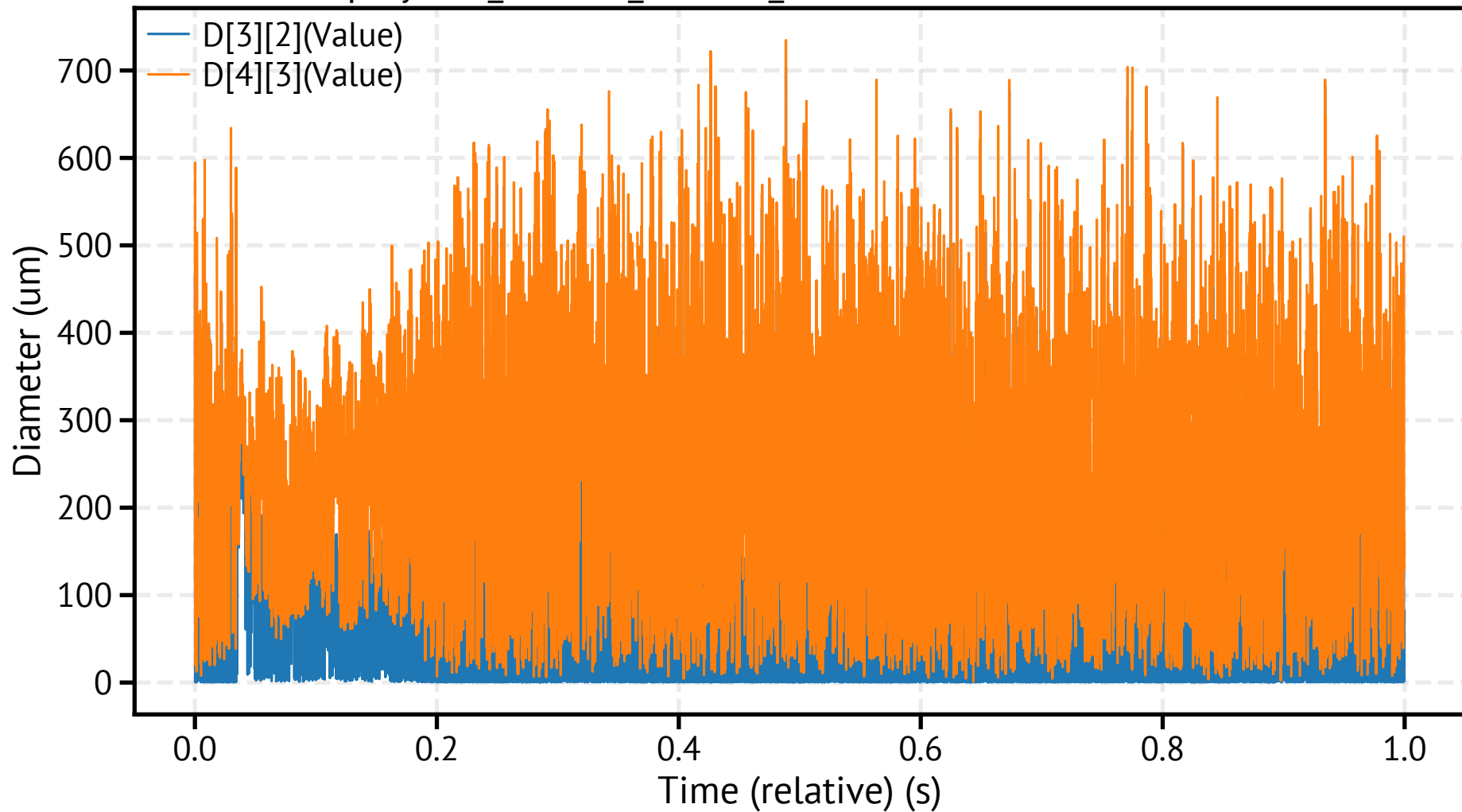
spraytec4_260310_170123_284600.csv - Mean Diameters
