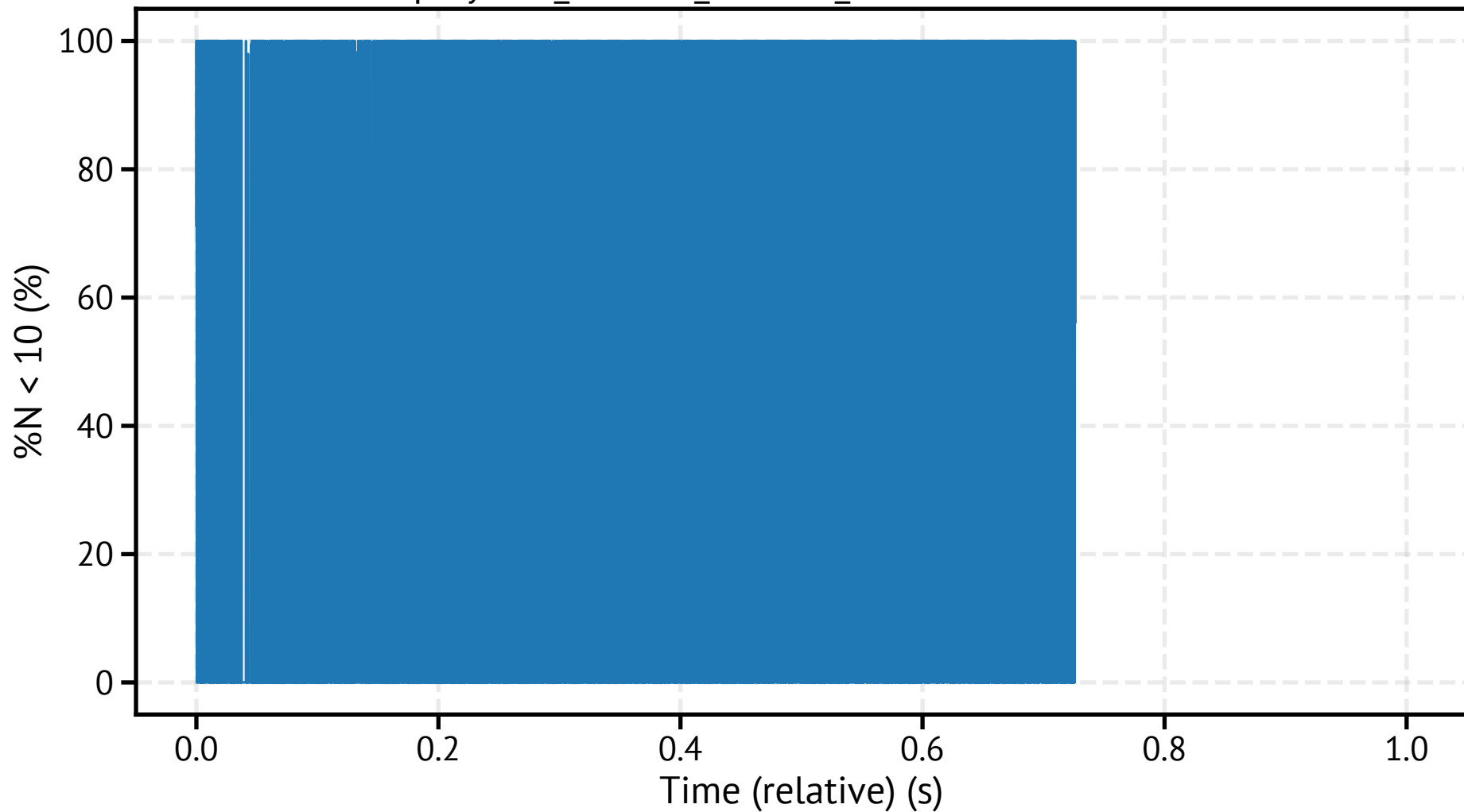
spraytec5_260310_170151_188800.csv - %N < 10
