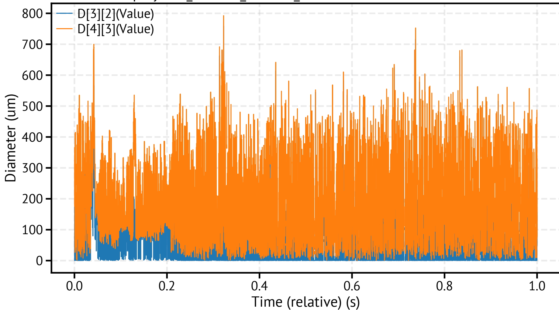
spraytec2_260311_151305_865100.csv - Mean Diameters
