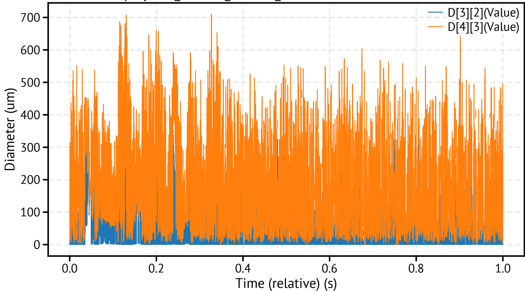
spraytec3_260311_151333_957000.csv - Mean Diameters
