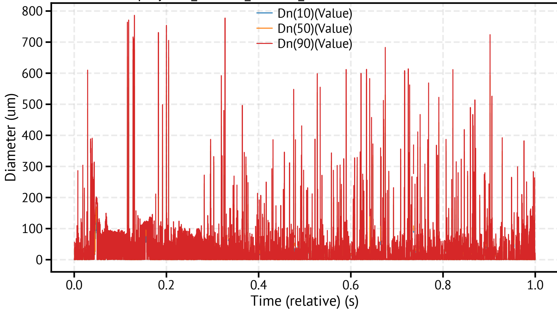
spraytec3_260311_151333_957000.csv - Dn Percentiles
