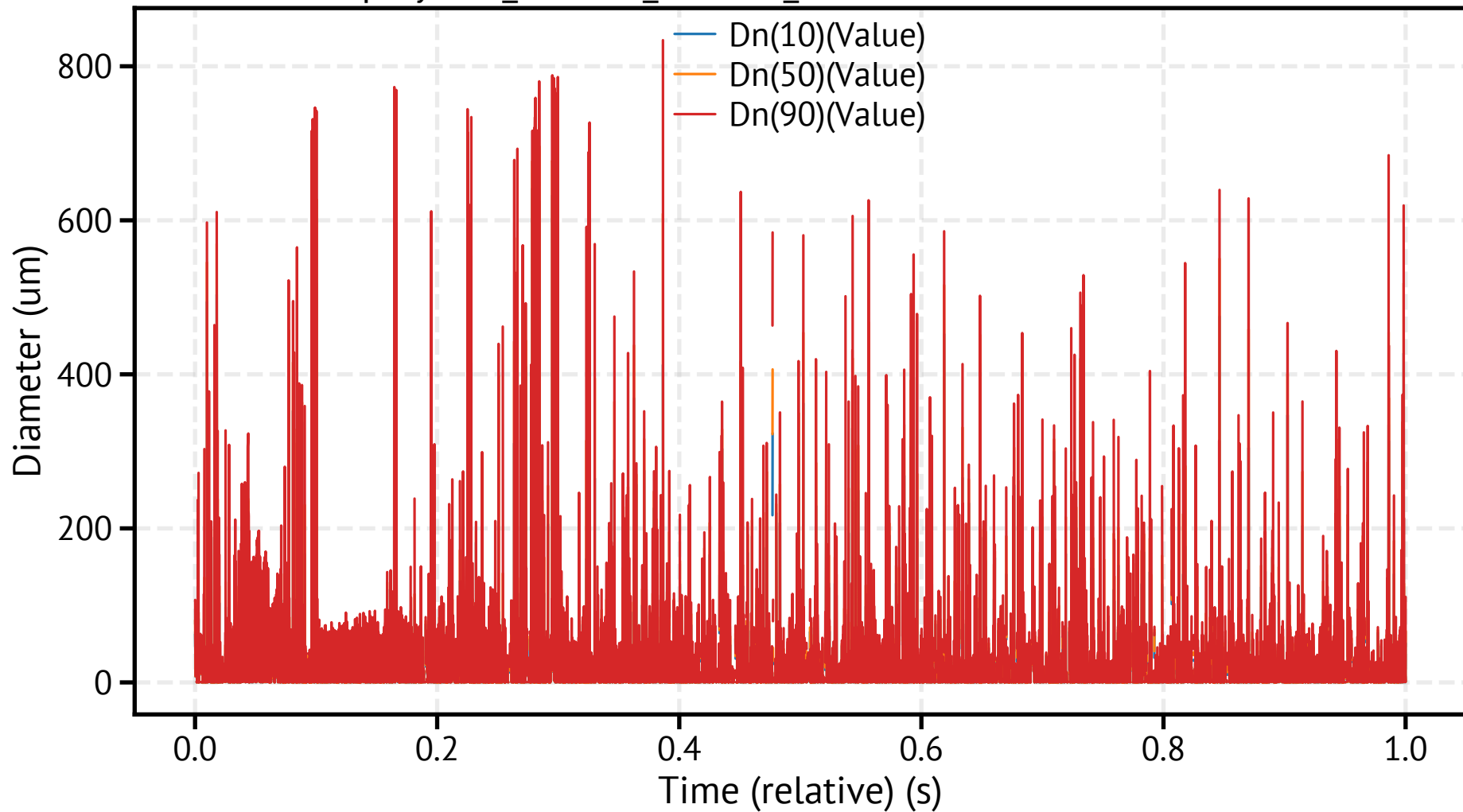
spraytec4_260311_151402_026700.csv - Dn Percentiles
