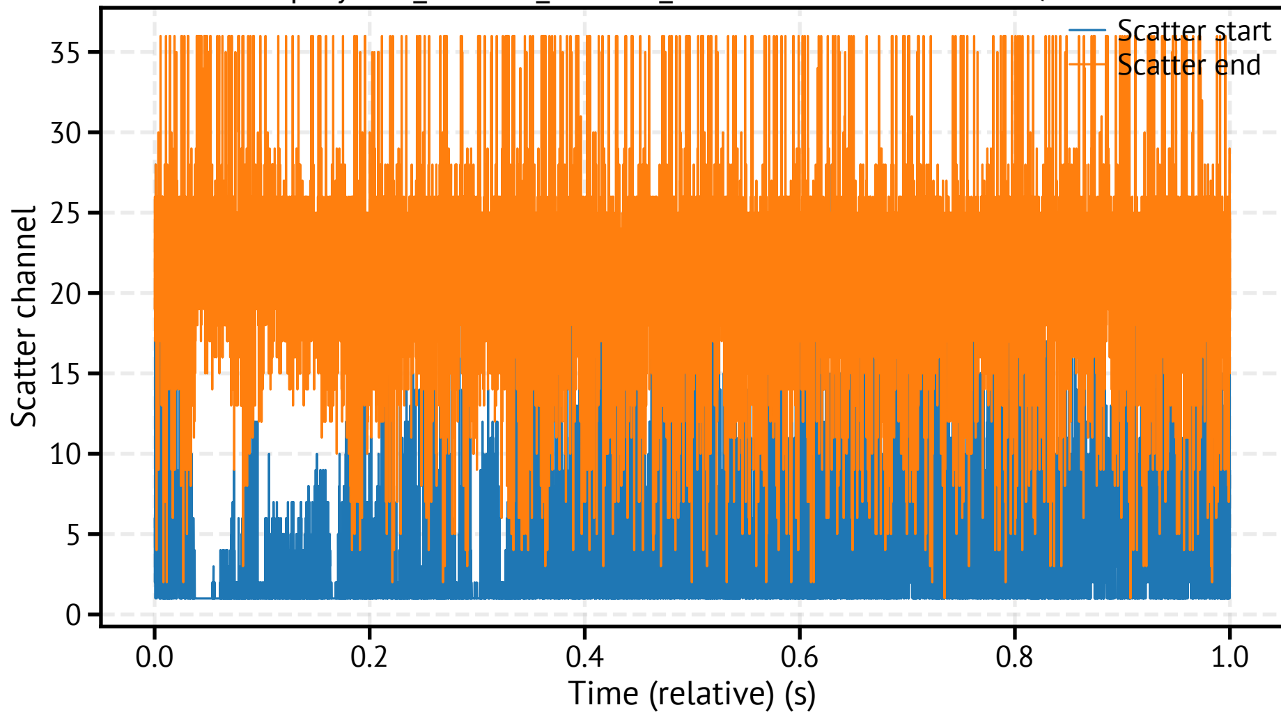
spraytec4_260311_151402_026700.csv - Scatter Start/End
