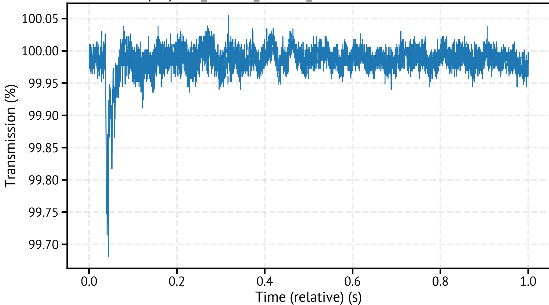
spraytec4_260311_151402_026700.csv - Transmission
