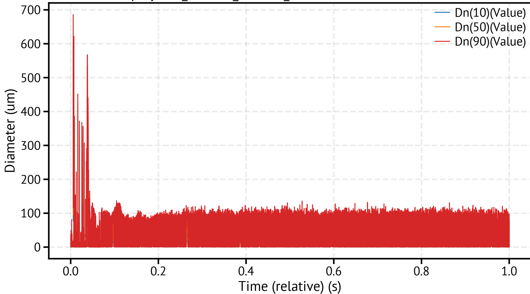
spraytec6_260311_151457_925300.csv - Dn Percentiles
