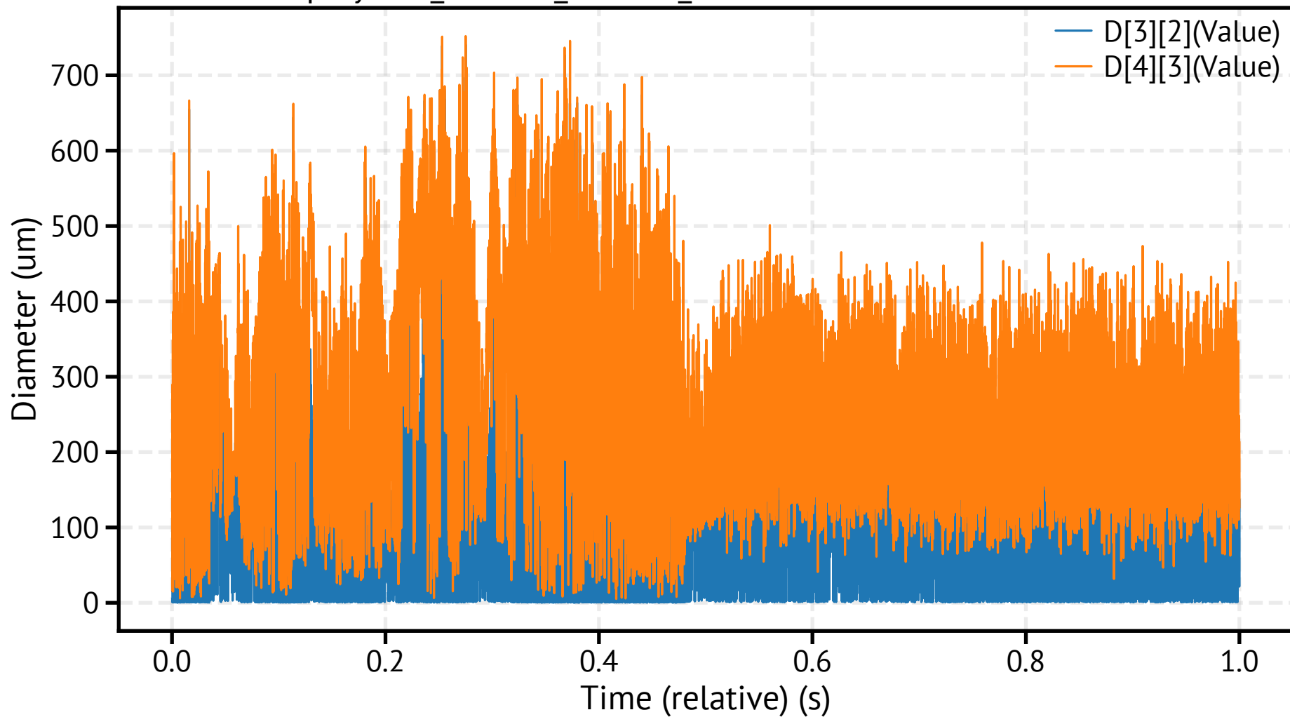
spraytec1_260311_153030_335900.csv - Mean Diameters
