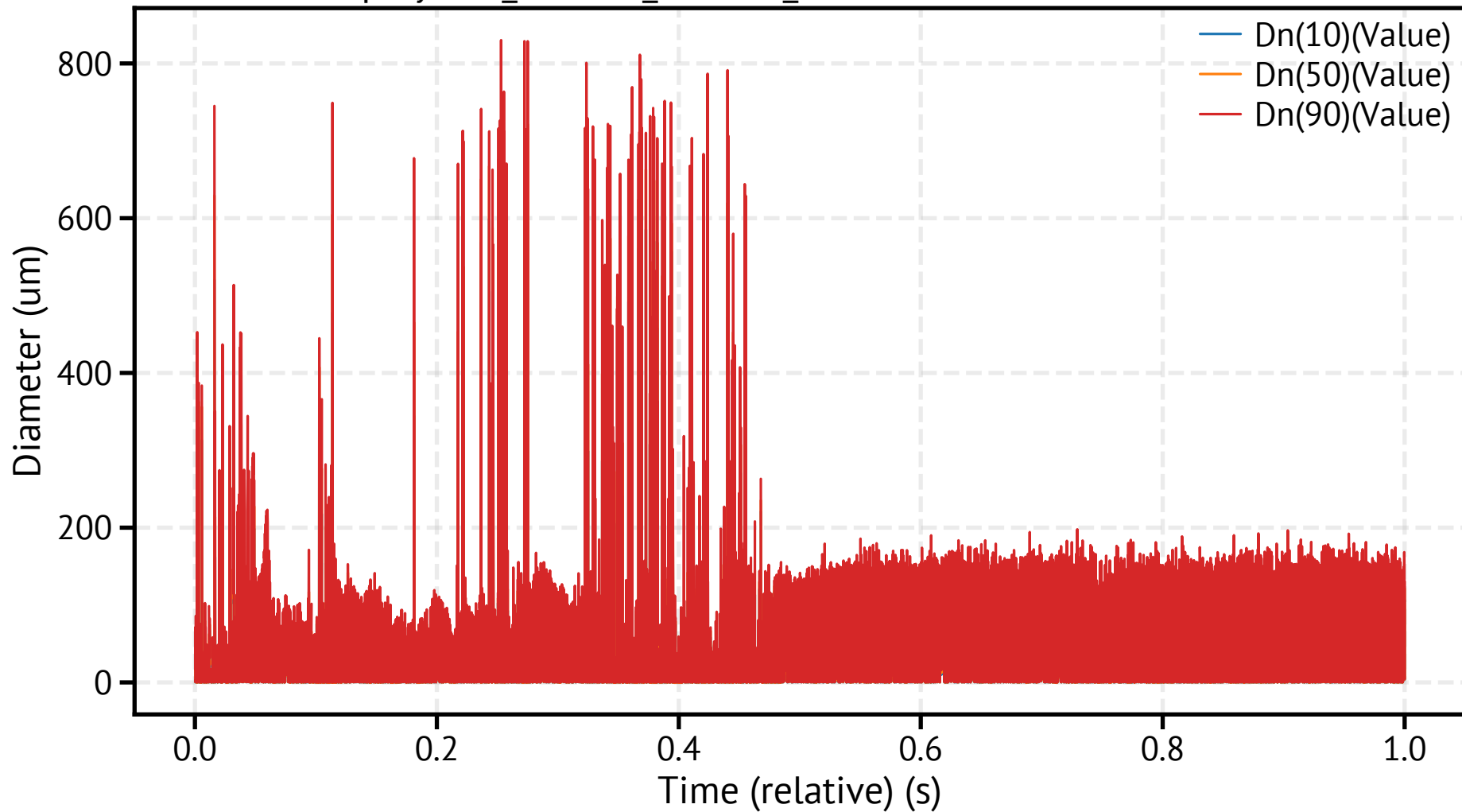
spraytec1_260311_153030_335900.csv - Dn Percentiles
