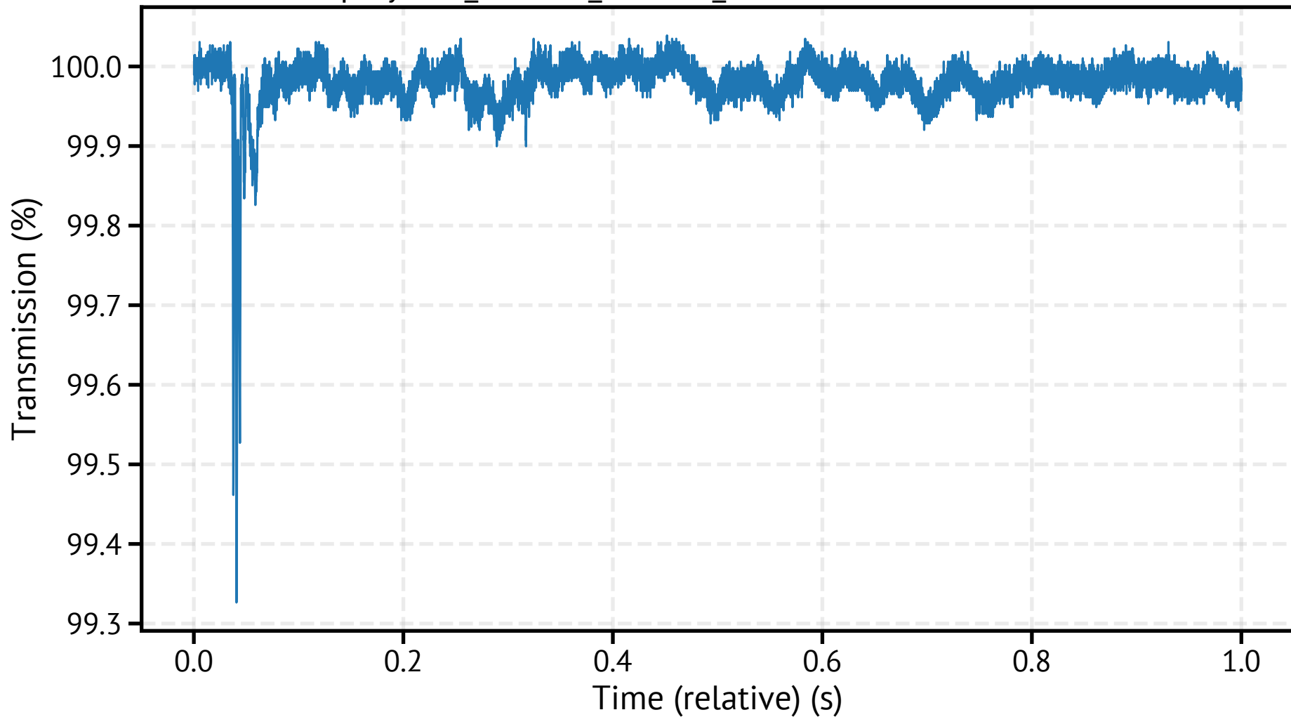
spraytec1_260311_153030_335900.csv - Transmission
