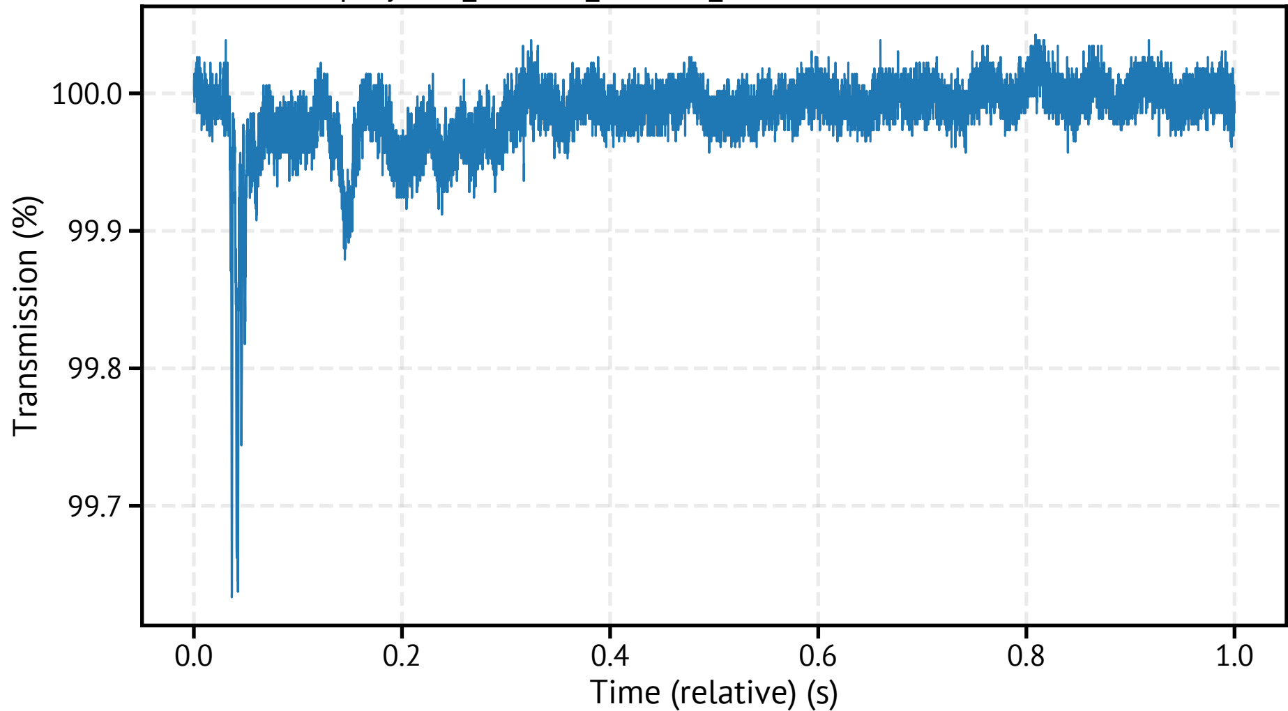
spraytec2_260311_153058_301400.csv - Transmission
