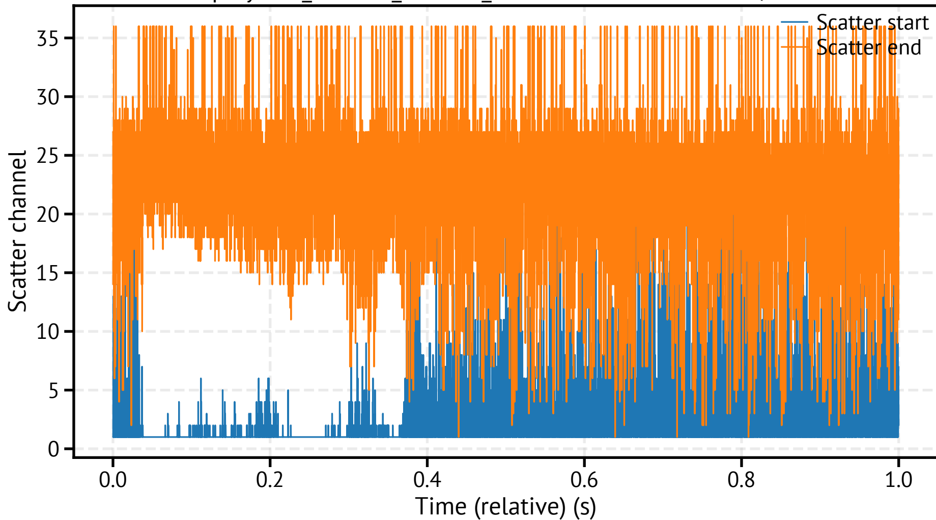
spraytec3_260311_153126_397100.csv - Scatter Start/End
