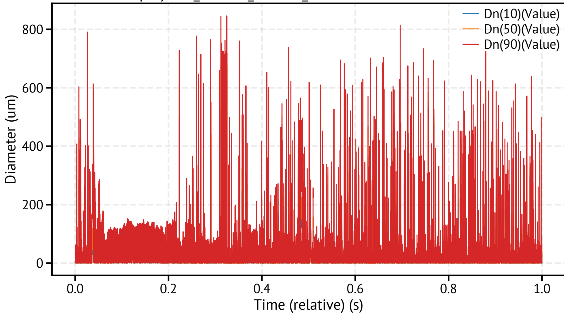
spraytec5_260311_153222_378700.csv - Dn Percentiles
