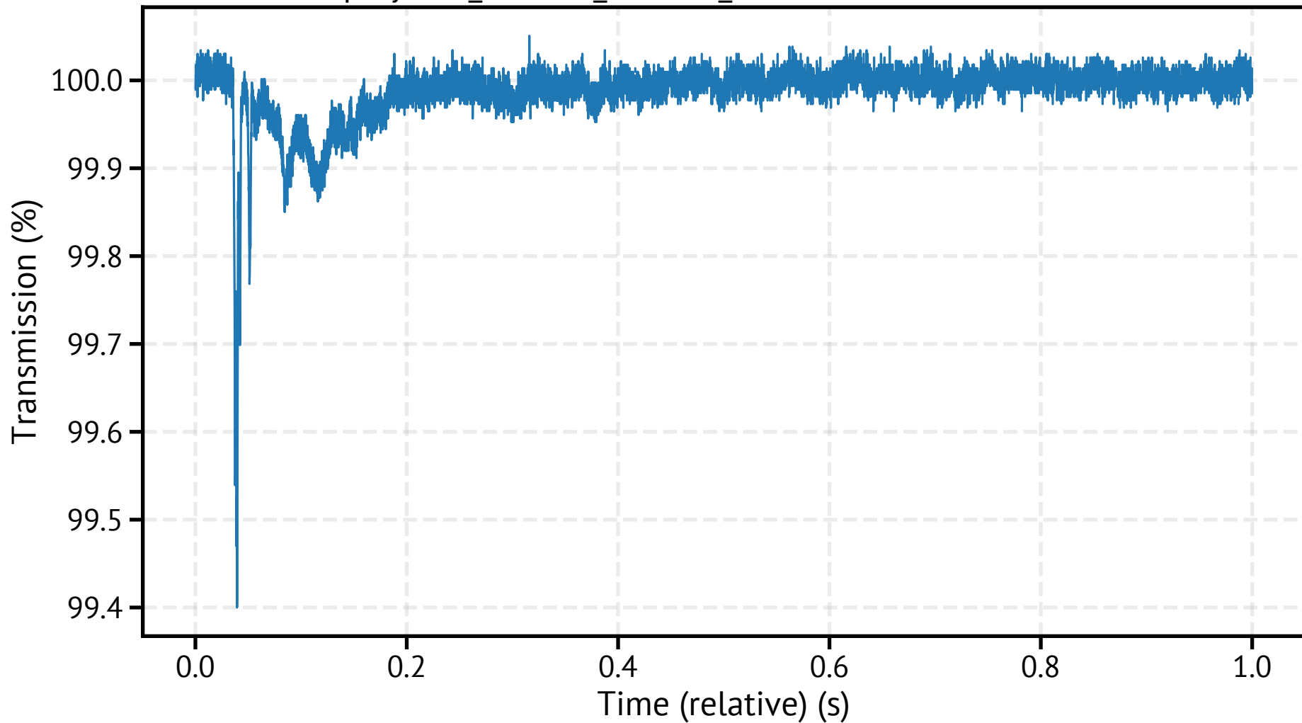
spraytec5_260311_153222_378700.csv - Transmission
