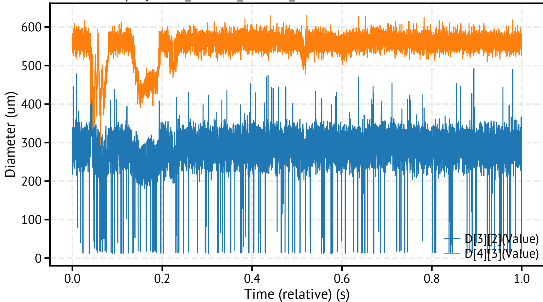
spraytec10_260318_100106_555800.csv - Mean Diameters
