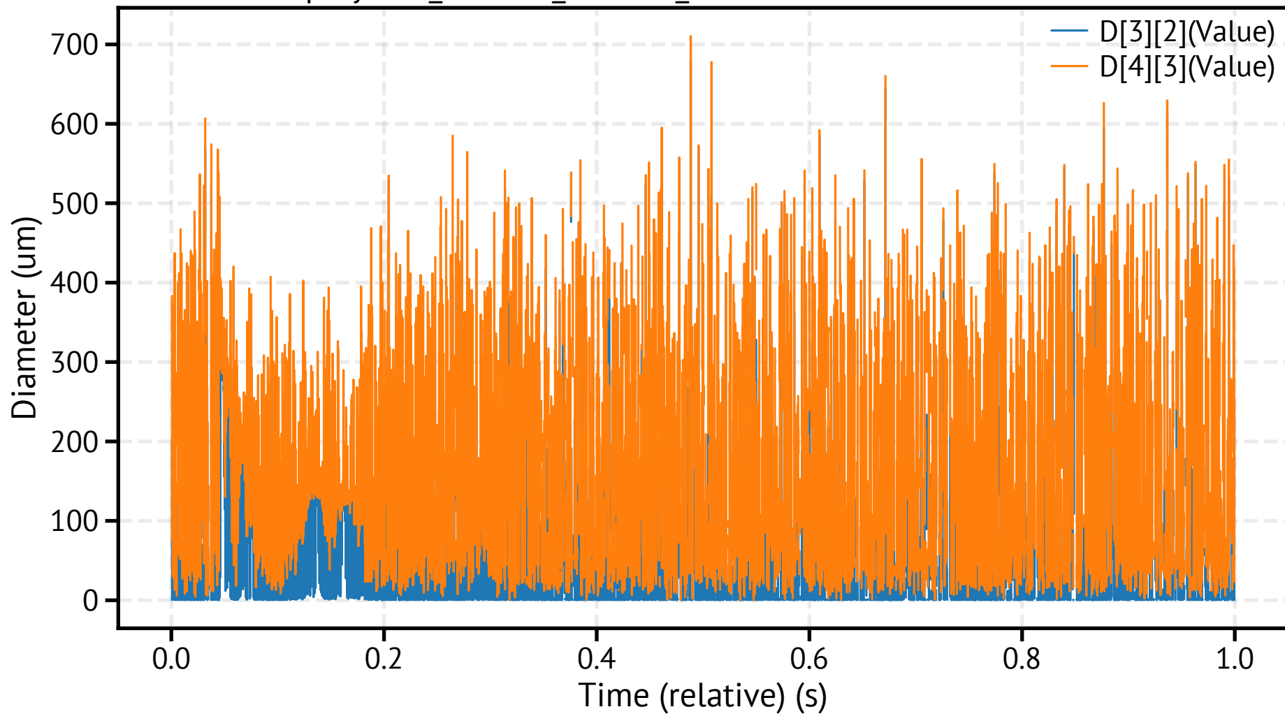
spraytec1_260318_095228_714300.csv - Mean Diameters
