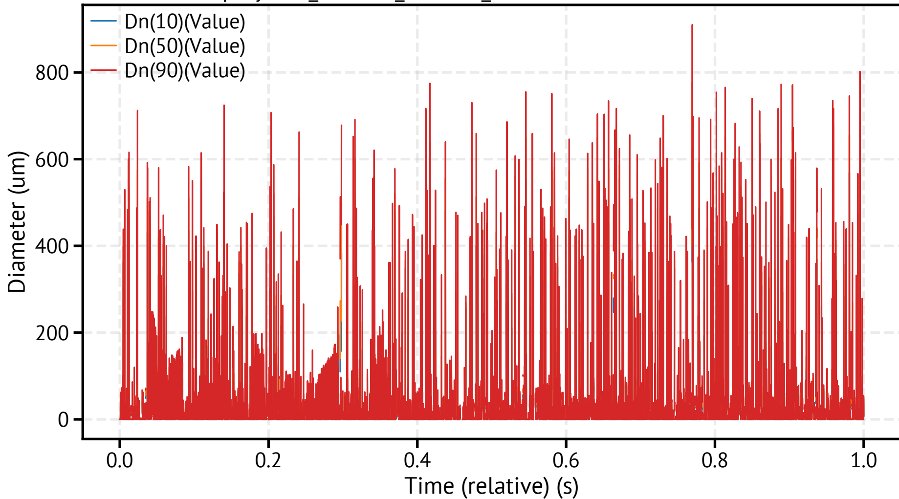
spraytec4_260318_095521_208200.csv - Dn Percentiles
