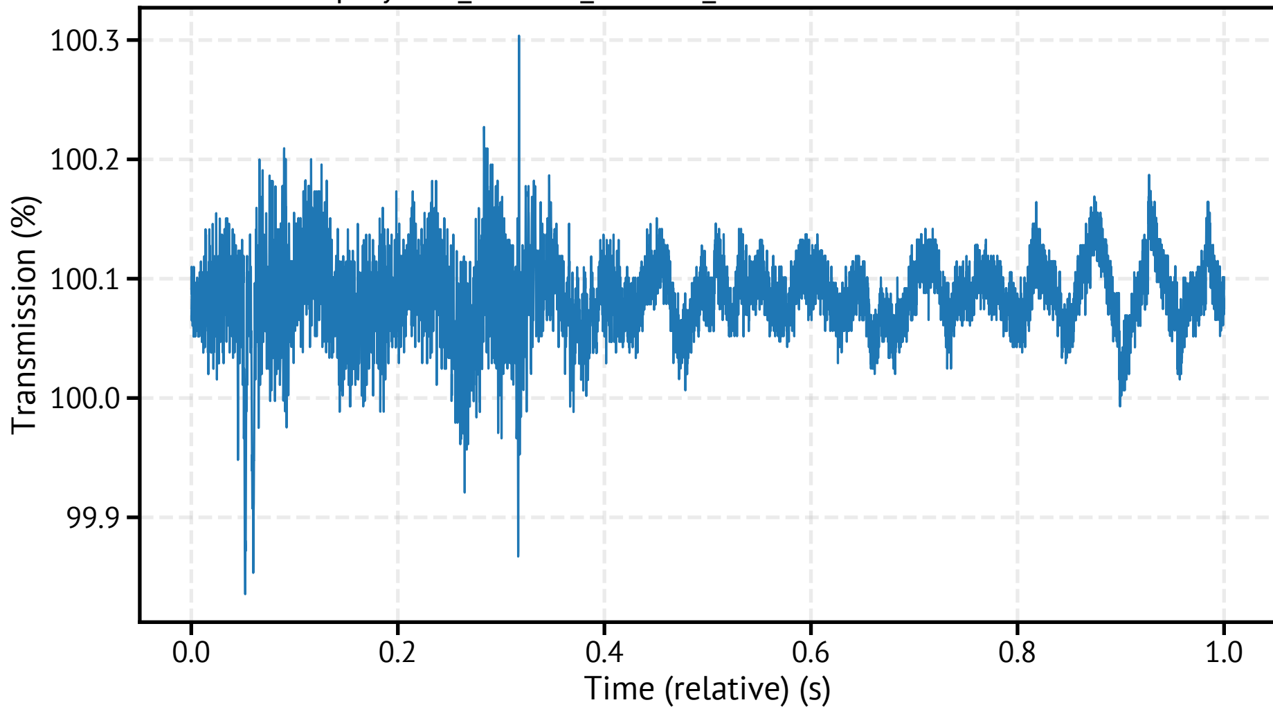
spraytec9_260318_100008_942700.csv - Transmission
