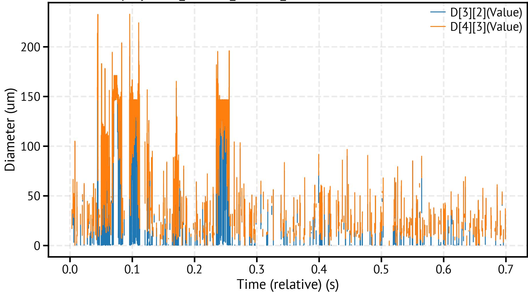
spraytec10_260318_103142_338800.csv - Mean Diameters
