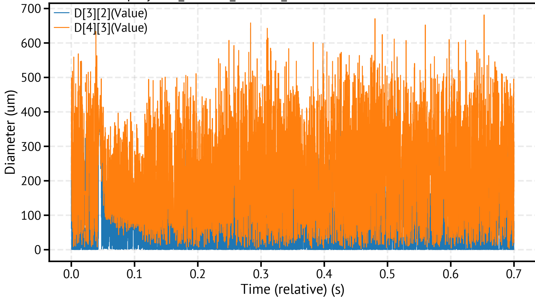
spraytec1_260318_103820_294500.csv - Mean Diameters
