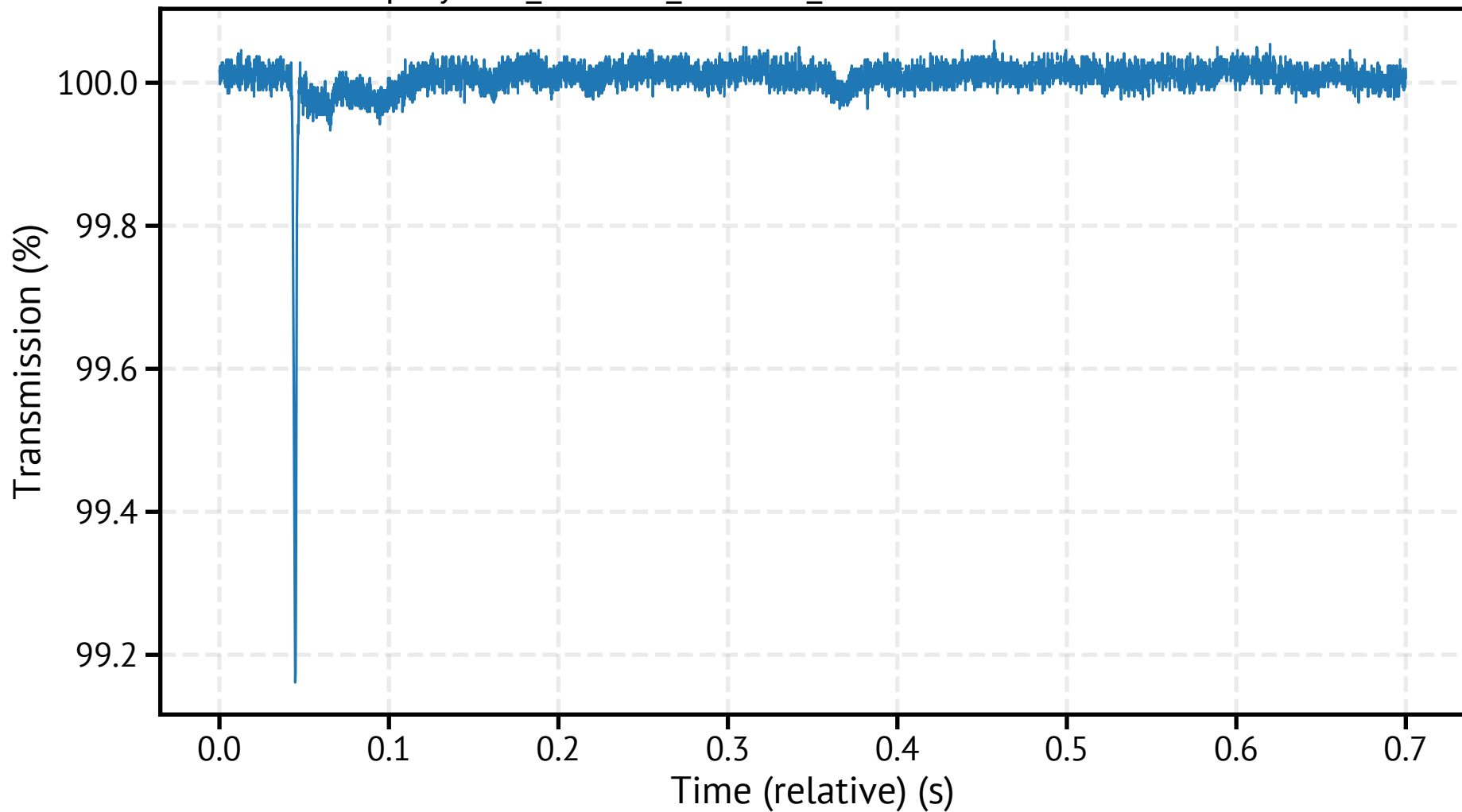
spraytec1_260318_103820_294500.csv - Transmission
