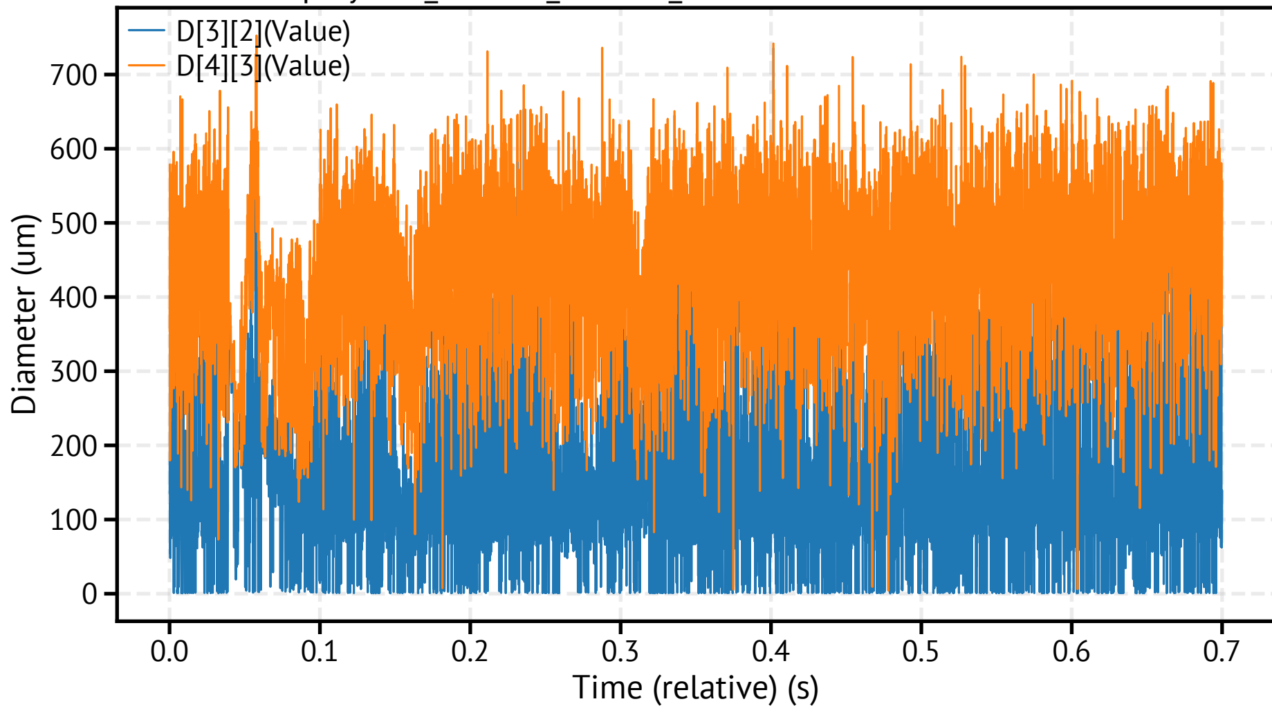
spraytec4_260318_104113_253000.csv - Mean Diameters
