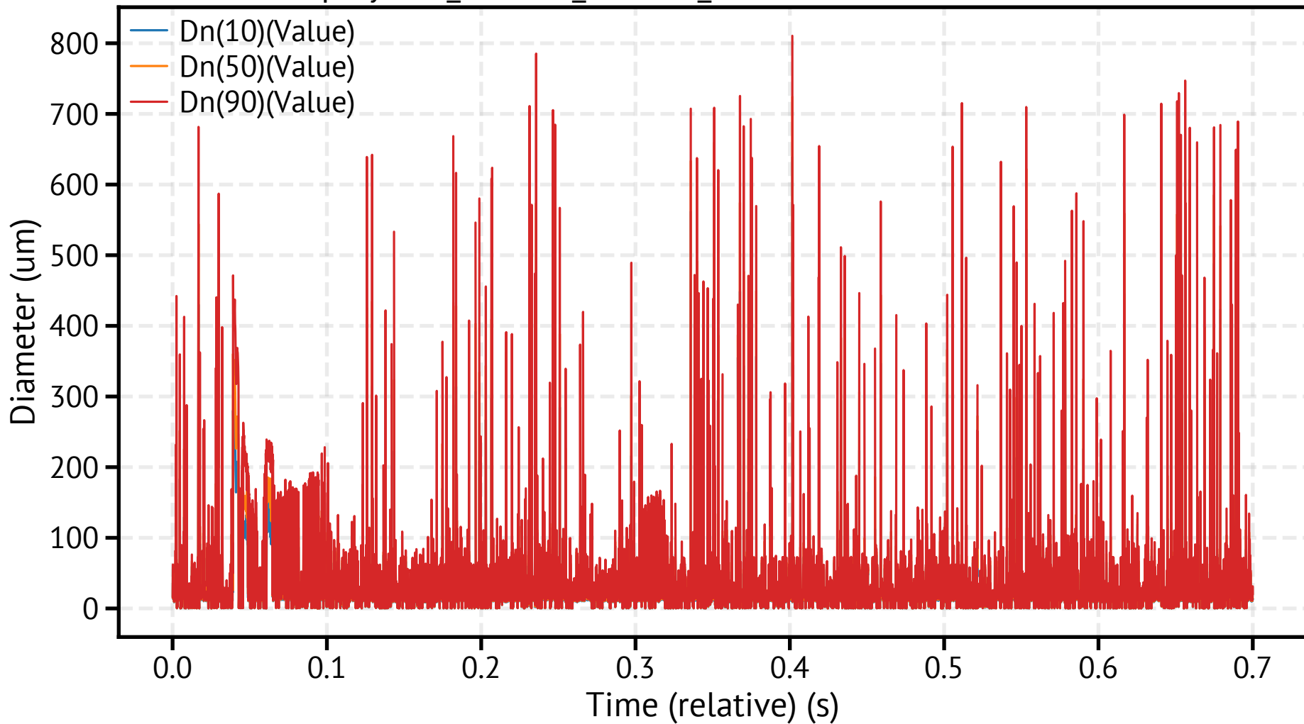
spraytec4_260318_104113_253000.csv - Dn Percentiles
