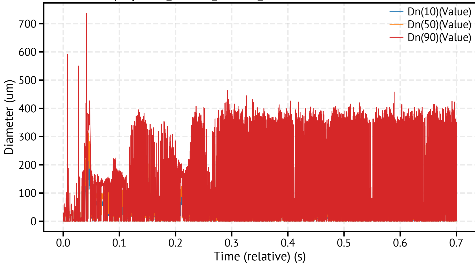
spraytec10_260318_111227_060600.csv - Dn Percentiles
