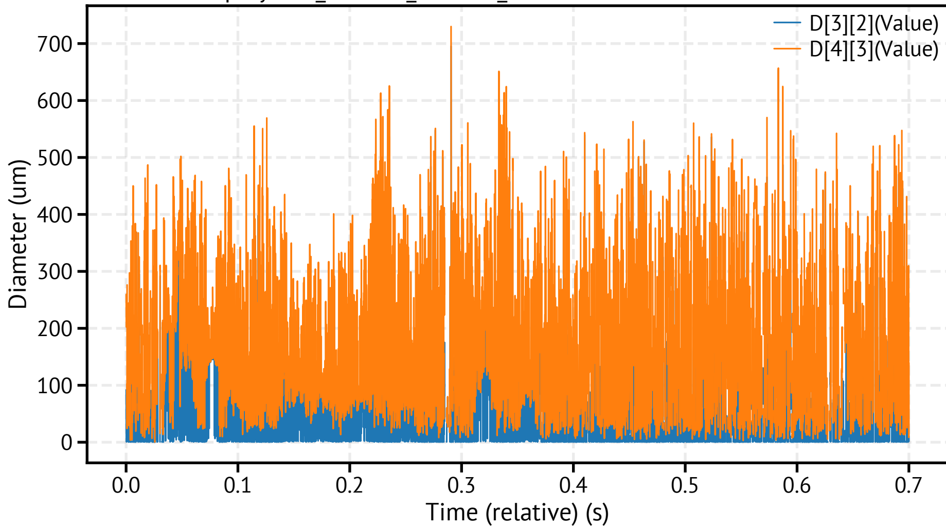
spraytec3_260318_110543_583400.csv - Mean Diameters
