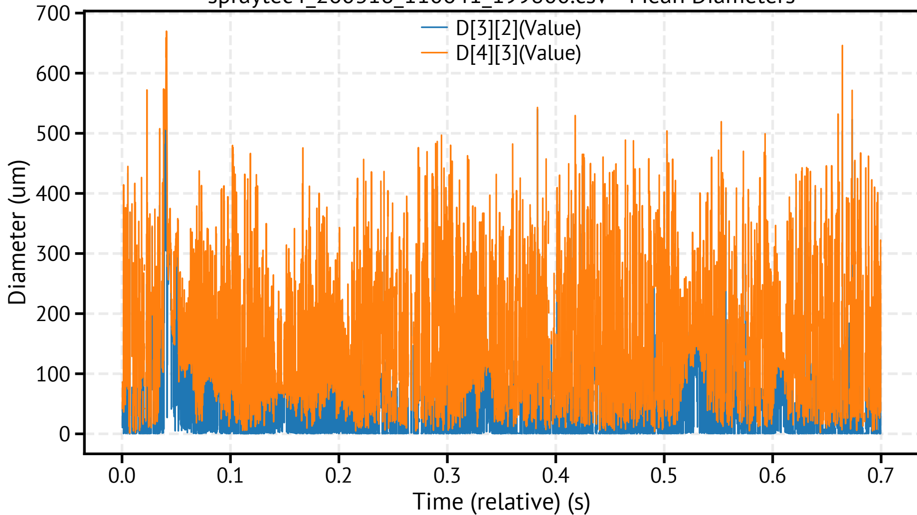
spraytec4_260318_110641_199800.csv - Mean Diameters
