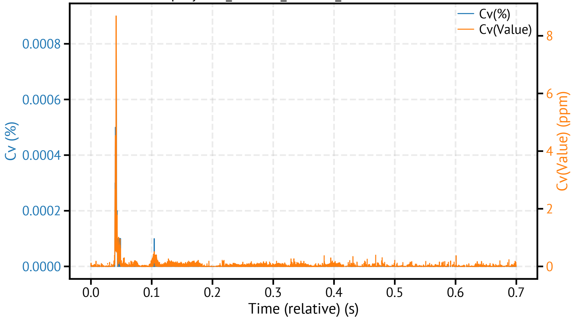
spraytec7_260318_110934_111900.csv - Cv
