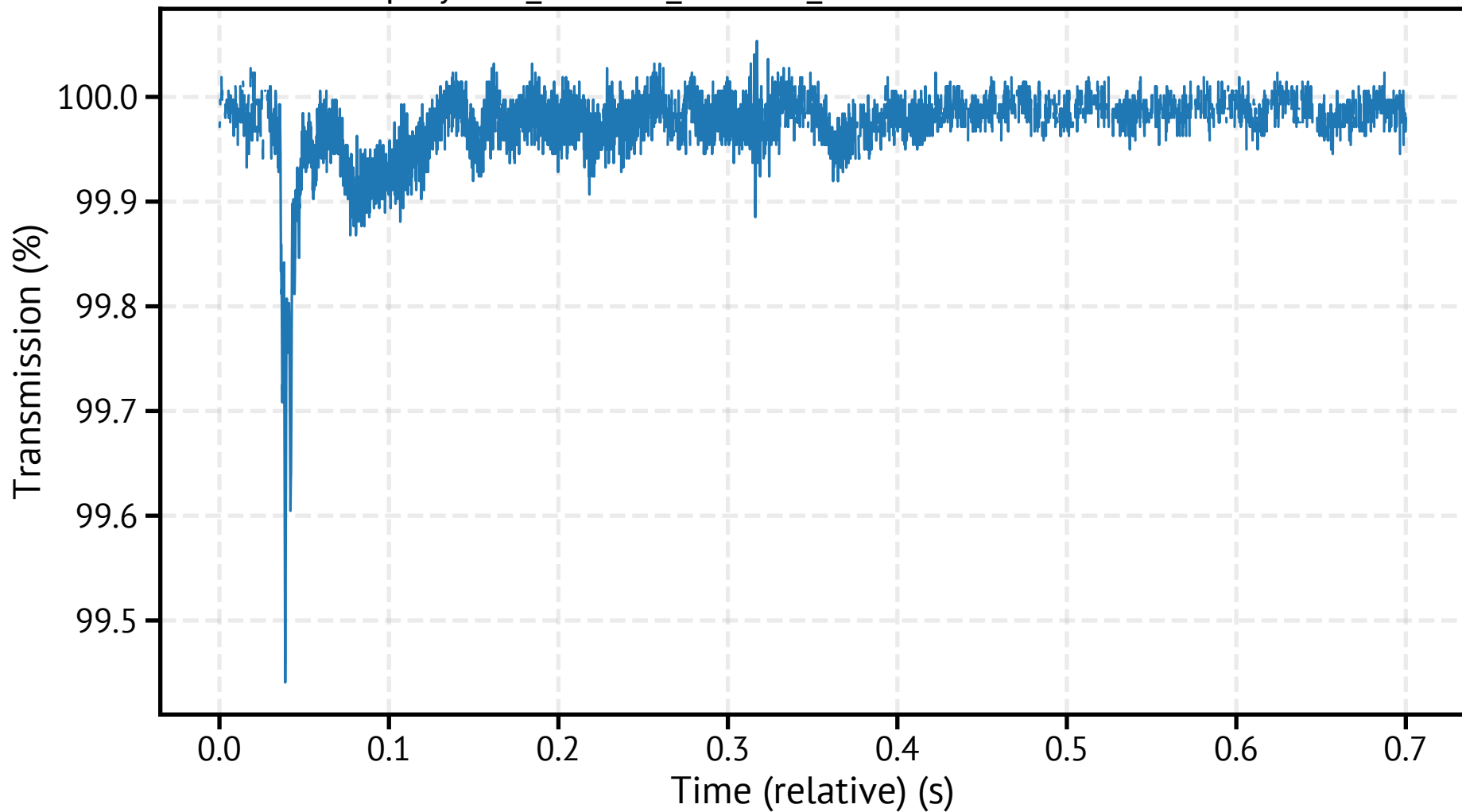
spraytec8_260318_111031_788900.csv - Transmission
