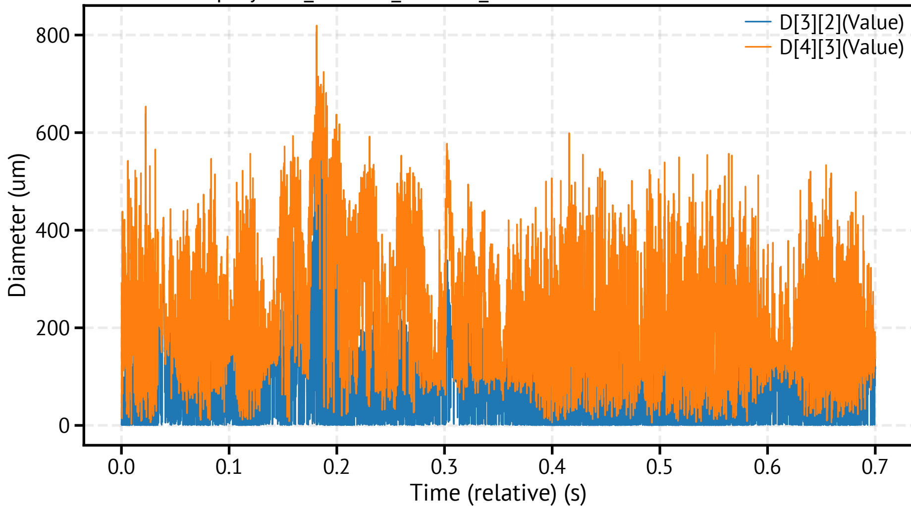
spraytec1_260318_111937_723200.csv - Mean Diameters
