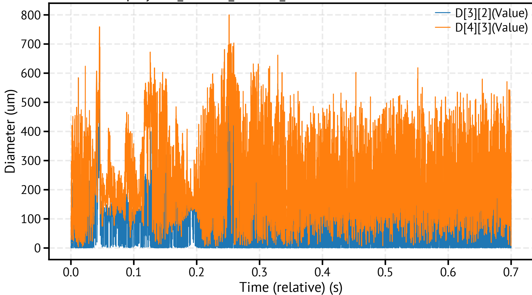
spraytec2_260318_112035_341900.csv - Mean Diameters
