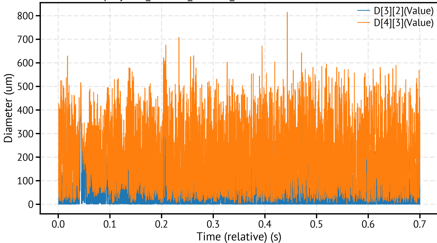
spraytec3_260318_112133_017200.csv - Mean Diameters
