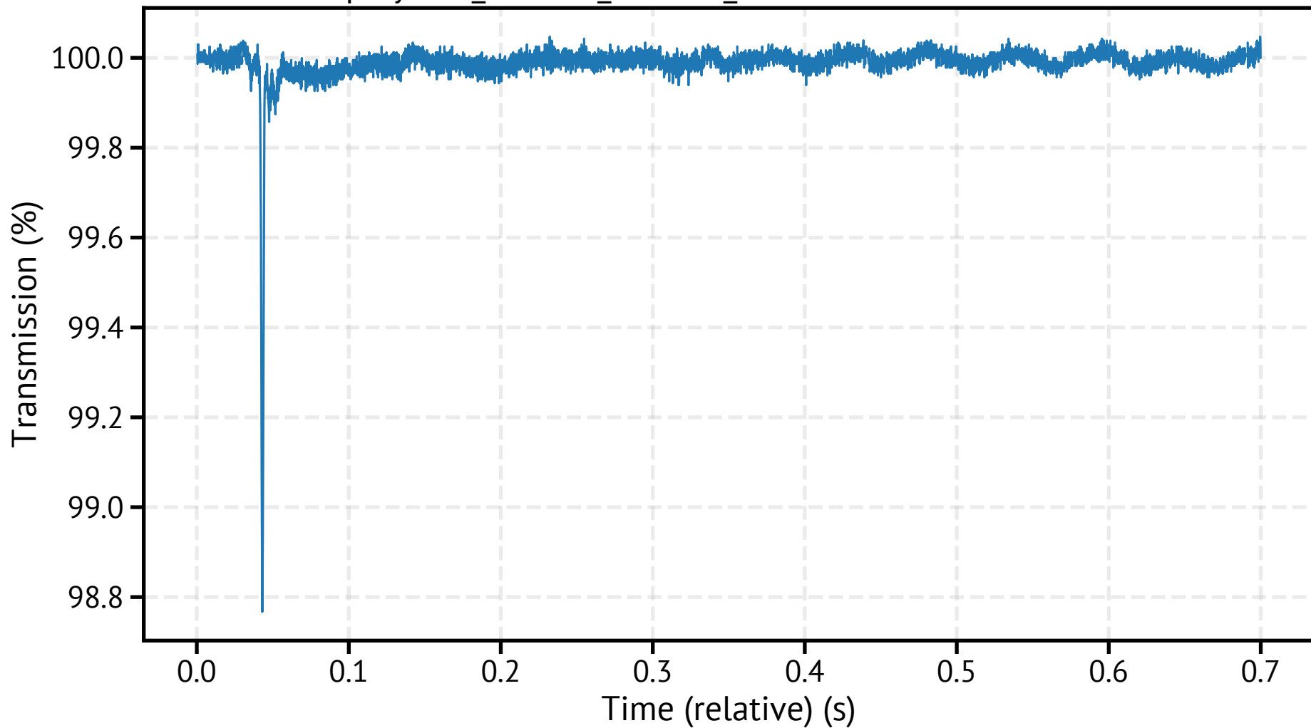
spraytec3_260318_112133_017200.csv - Transmission
