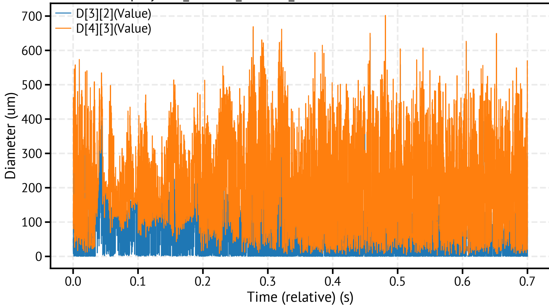
spraytec4_260318_112230_623100.csv - Mean Diameters
