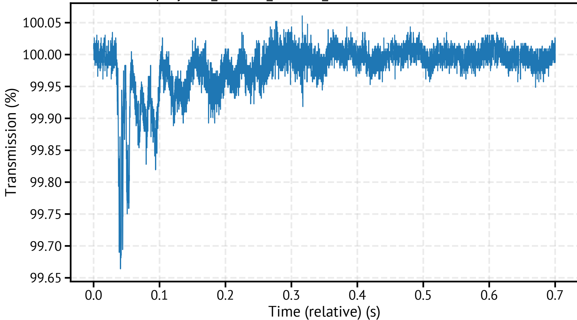
spraytec4_260318_112230_623100.csv - Transmission
